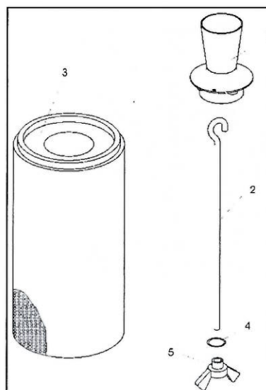
1: Venturi 2: Rod 3: Filter cartridge 4: Rod seal 5: Wing nut
